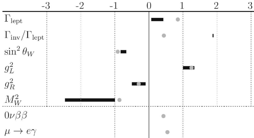
Figure 2: EWPOs calculated at the best-fit point for NH and suppressed \epsilon_\mu (light-gray dots) compared to the experimentally observed values, denoted by the zero line. The vertical lines stand for the respective experimental sigma deviations, thus the displacement of the predicted values from the observations is presented in units of the experimental error. Note that for the 0\nu\beta\beta and \mu \rightarrow e\gamma constraints we present only the one sigma exclusion limits. The theoretical predictions of the SM with their theoretical uncertainties are displayed as well (dark-gray bars). (The best-fit point is at M_1 = 20.3 TeV, M_2 = 14.1 TeV, M_3 = 21.0 TeV, \epsilon_e = 2.1 \cdot 10^{-3} , \epsilon_\mu = 3.0 \cdot 10^{-6} and \epsilon_\tau = 4.5 \cdot 10^{-3} .)
