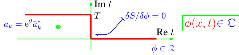
Figure 2: Semiclassical boundary value problem.
