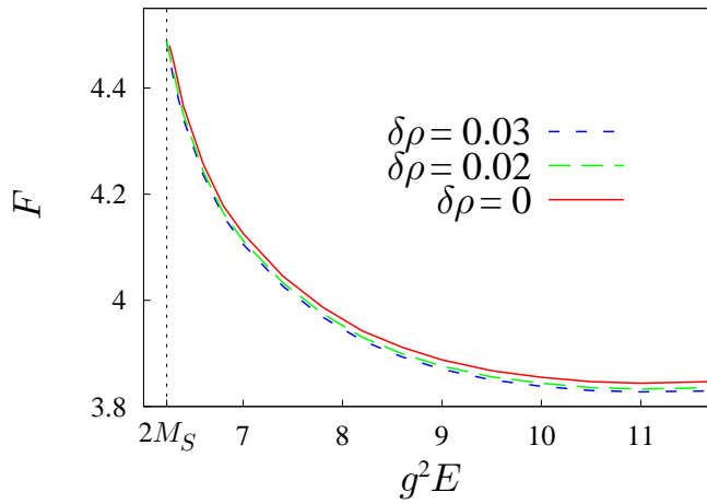
Figure 5: Two-particle suppression exponents F(E) at different \delta\rho .
