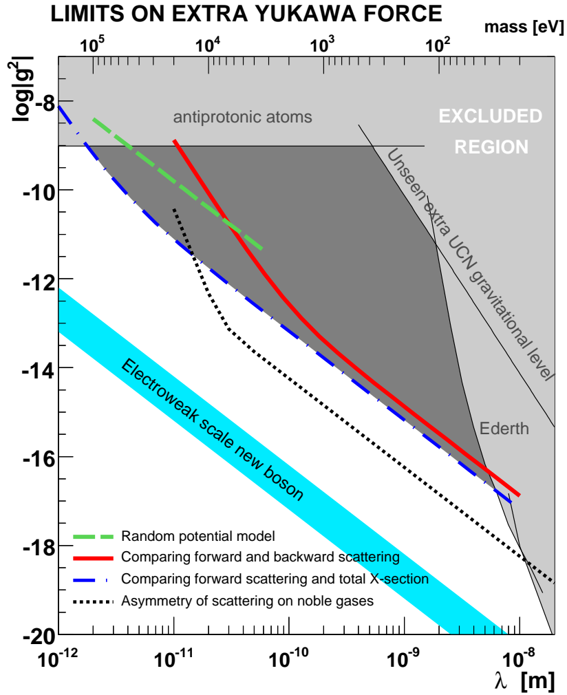
Figure 1: The shaded regions correspond to current experimental limits on extra Yukawa interaction. It includes constraint at 95 % C.L. (dashed, dot-dashed and bold lines) obtained in this article, and the existing constraints [11, 13]. The dotted line is an estimation of the sensitivity of proposed experiment.
