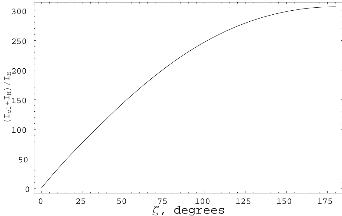
Figure 2: The amplification of the annihilation signal (I_{\text{cl}} + I_{\text{H}})/I_{\text{H}} as function of the angle between the line of observation and the direction to the Galactic center.
