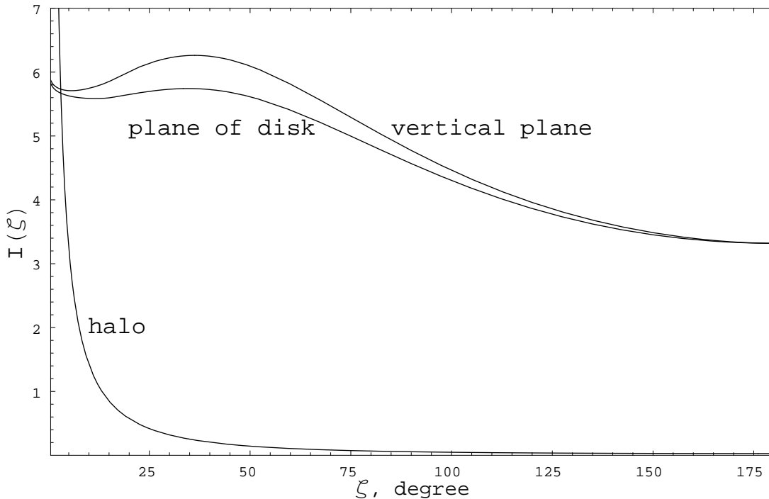
Figure 3: The annihilation signal in the Galactic disk plane and in vertical plane.
