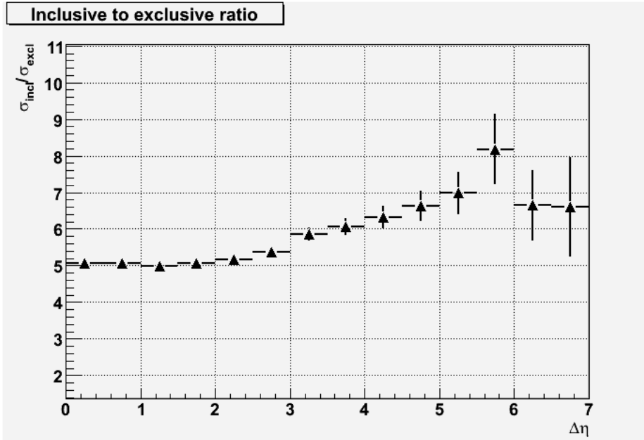
Figure 1: Dijet K-factor at LHC: inclusive dijet cross section over only-two-jet cross section ratio. The results are shown with full CMS detector simulation (arbitrary normalization) for luminosity pb^{-1} .
