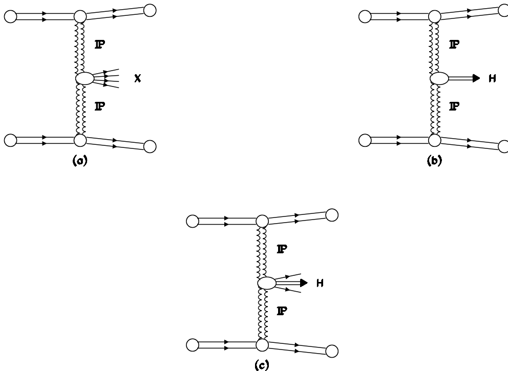
Figure 1: The double-diffractive processes for production in central region via double-Pomeron exchange: (a) double-Pomeron exchange for inelastic central production; (b) exclusive central Higgs boson production; (c) inclusive central inelastic Higgs boson production
