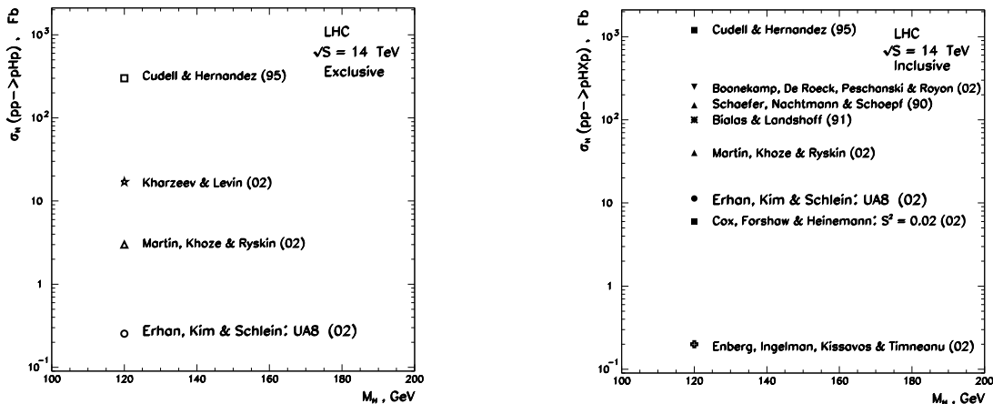
Figure 4: Comparison of the predictions for the LHC, based on UA8 data, with available calculations for: (a) exclusive and (b) inclusive cross sections
