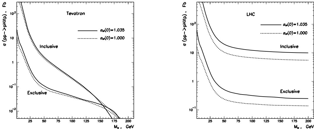
Figure 2: The cross section of exclusive pp \rightarrow pHp and inclusive pp \rightarrow pHXp double-diffractive Higgs boson production suggested by UA8 data for: (a) the Tevatron and (b) the LHC
