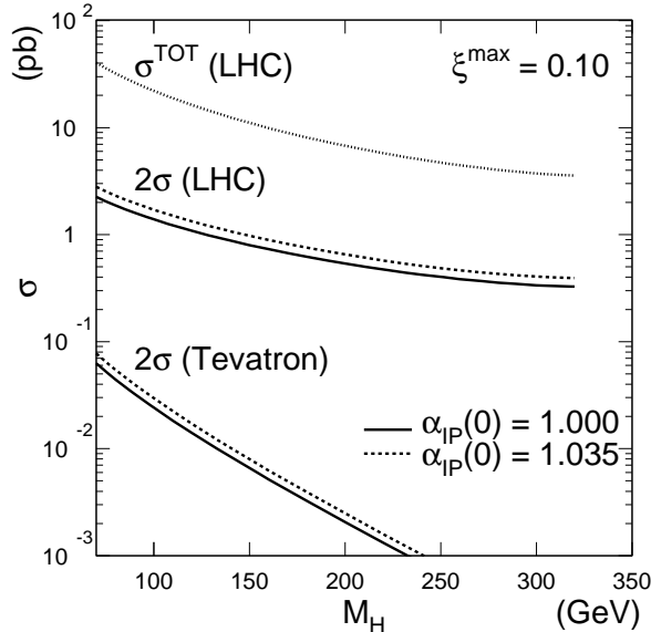
Figure 7: The predictions for inclusive single-Pomeron exchange cross section at Tevatron and LHC energies based on UA8 data.
