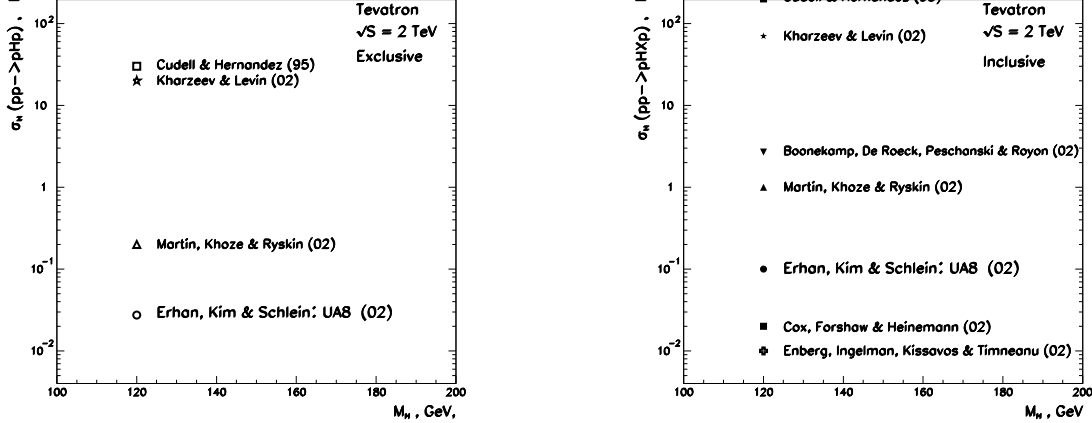
Figure 3: Comparison of the predictions for the Tevatron, based on UA8 data, with available calculations for: (a) exclusive and (b) inclusive cross sections
