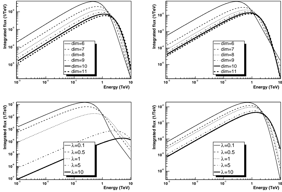
Figure 1: Integrated flux as a function of the total energy of the emitted quanta for an initial black hole mass M = 10 TeV. Upper left: \lambda = 0 , D = 6, 7, 8, 9, 10, 11 . Upper right : \lambda = 0,5 \text{ TeV}^{-2} , D = 6, 7, 8, 9, 10, 11 . Lower left : D = 6 , \lambda = 0.1, 0.5, 1, 5, 10 \text{ TeV}^{-2} . Lower right : D = 11 , \lambda = 0.1, 0.5, 1, 5, 10 \text{ TeV}^{-2} .
