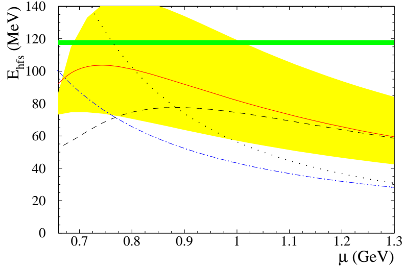
Figure 2: HFS of 1S charmonium as a function of the renormalization scale \mu in the LO (dotted line), NLO (dashed line), LL (dot-dashed line), and NLL (solid line) approximations. For the NLL result, the band reflects the errors due to \alpha_s(M_Z) = 0.118 \pm 0.003 . The horizontal band gives the experimental value 117.7 \pm 1.3 MeV [25].
